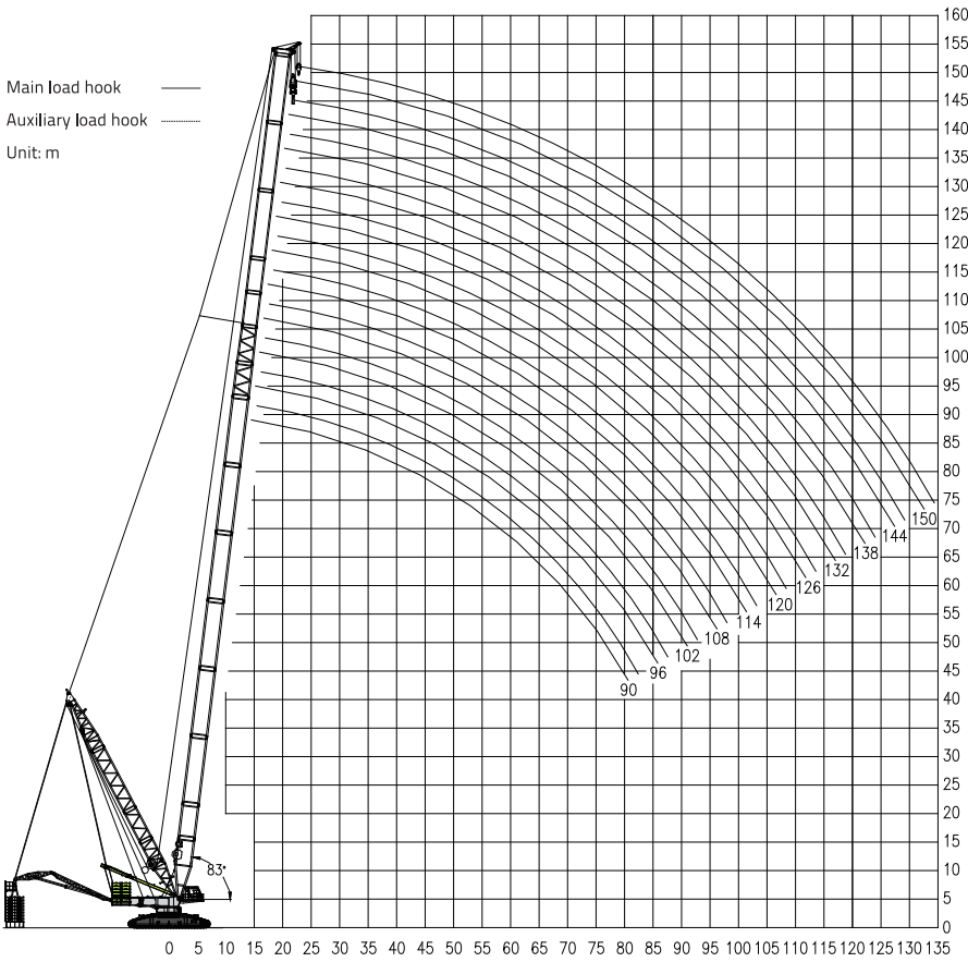
4.2 Hoisting height curves and lifting capacity charts of SLDB-1
