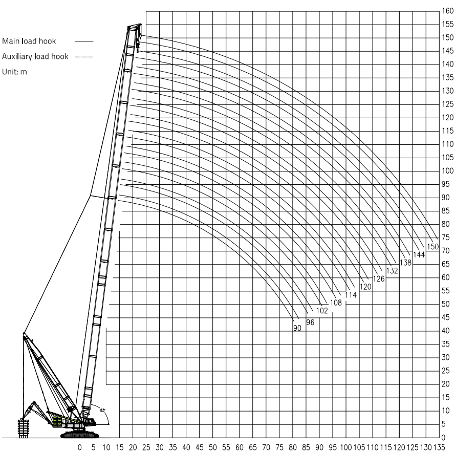
4.3 Hoisting height curves and lifting capacity charts of SLPDB-1
