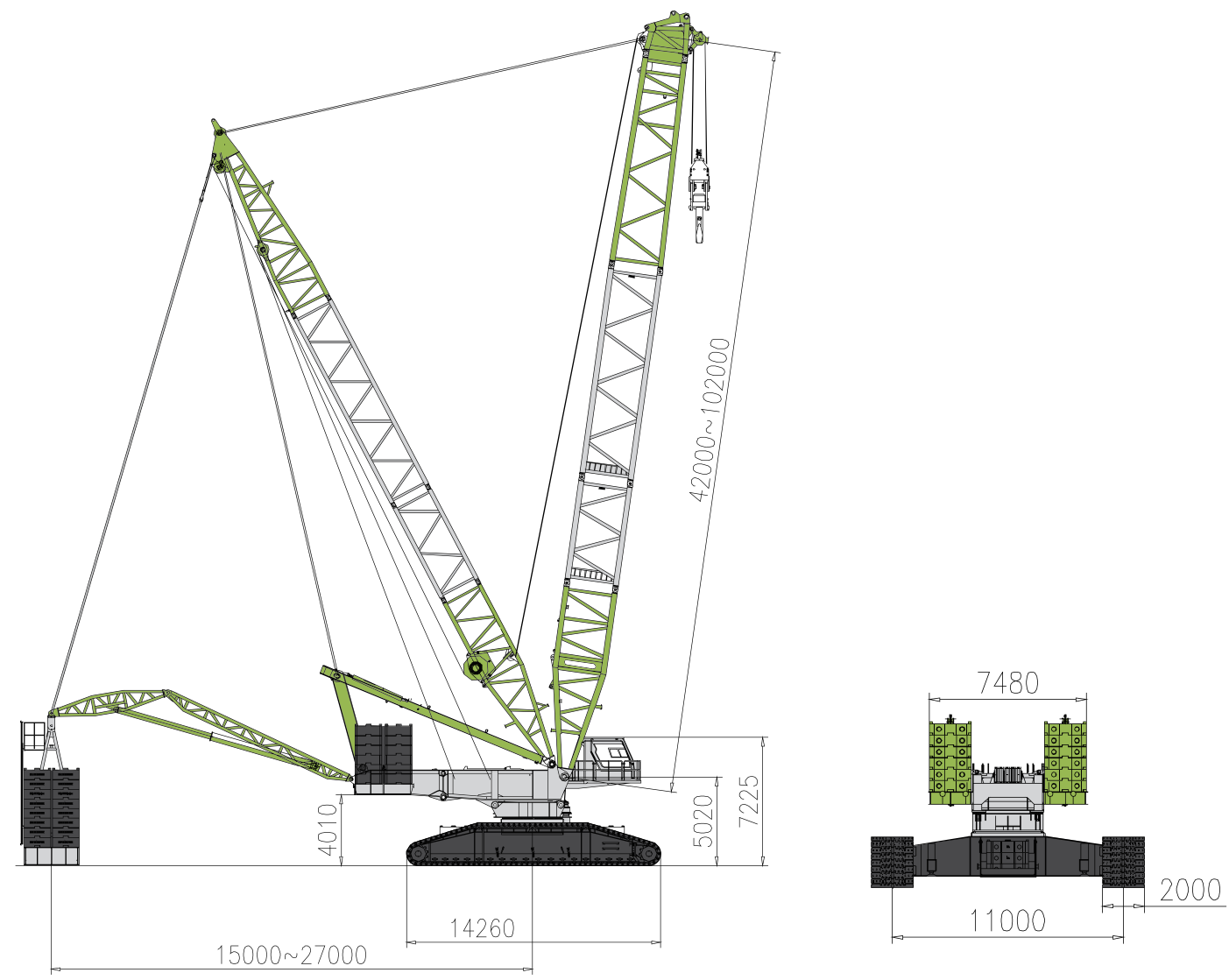
Overall dimensions of SDB mode
