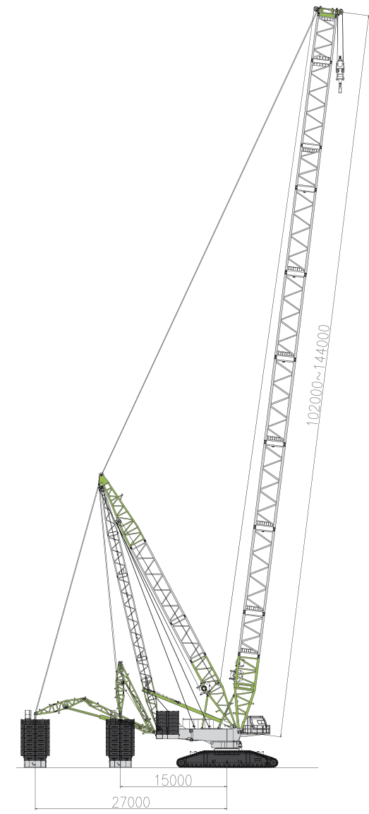
Overall dimensions of SLDB-2 mode
