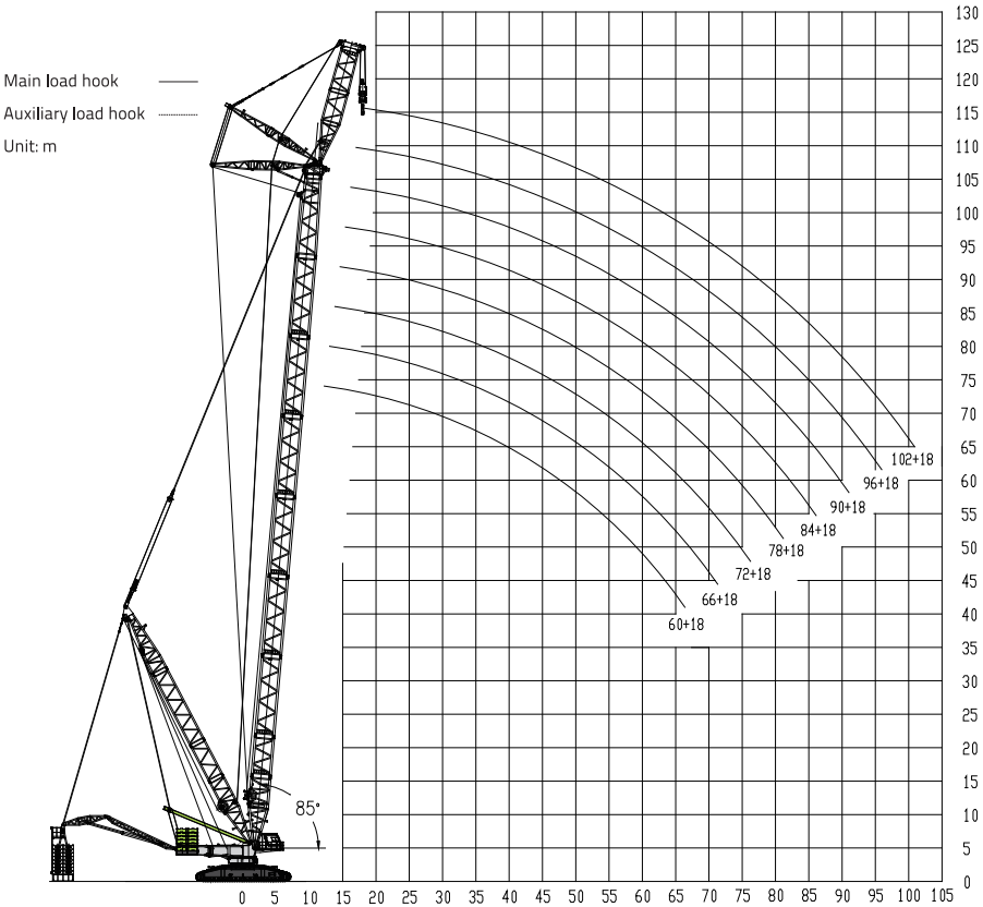
4.8 Hoisting height curves and lifting capacity charts of SFVDB
