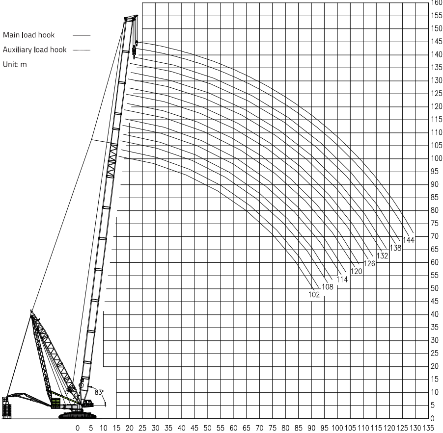
4.4 Hoisting height curves and lifting capacity charts of offshore wind power SLDB-2
