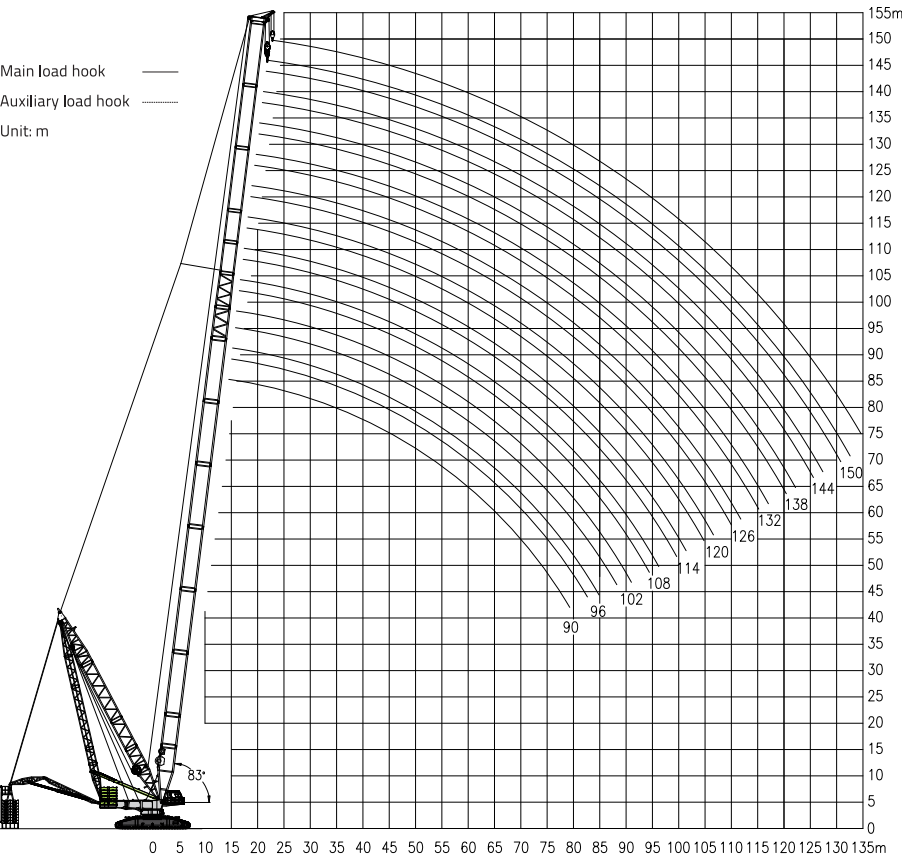
4.5 Lifting capacity charts of SLDB-3 /SLPDB-2/3
