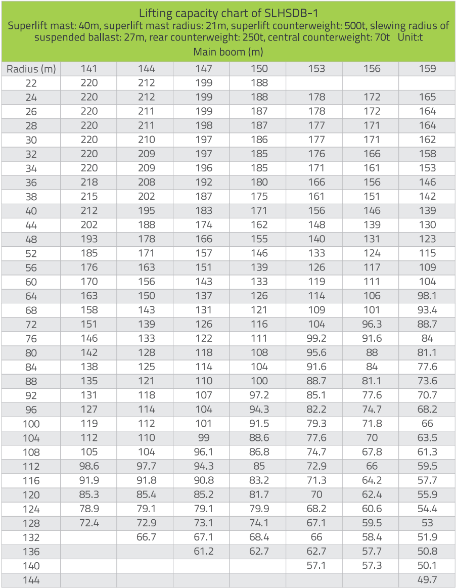
4.6 Lifting capacity charts of SLHSDB-1
