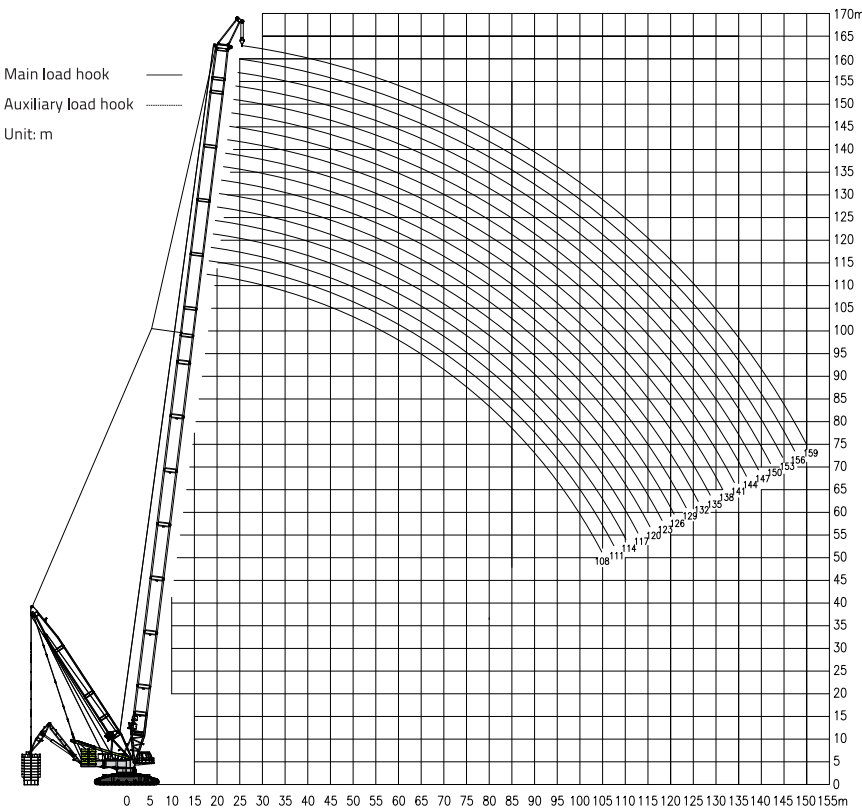
4.6 Hoisting height curves and lifting capacity charts of SLHSDB-1
