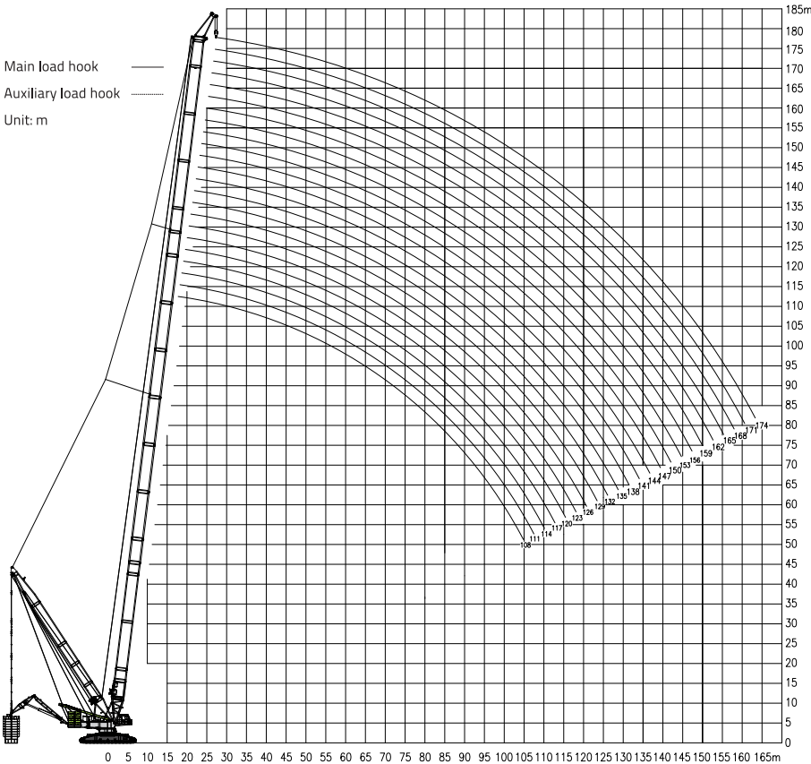
4.7 Hoisting height curves and lifting capacity charts of SPHSDB-1 / SPHSDB-2
